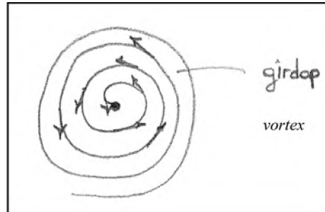
Figure 4(a). Student 1's diagram for the curl of flow velocity of a moving fluid
